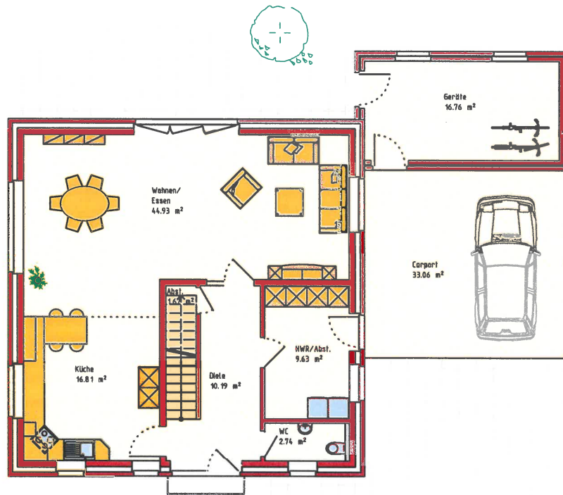
Erdgeschoss WF 85.97 m 2
